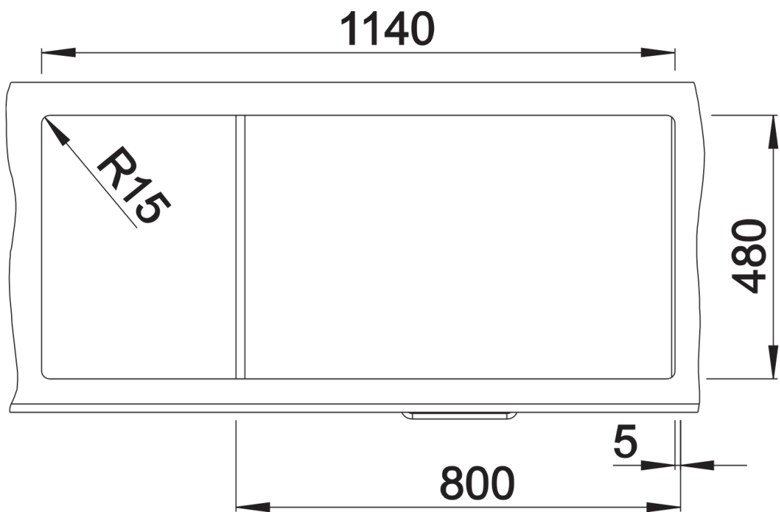
Cut-out
